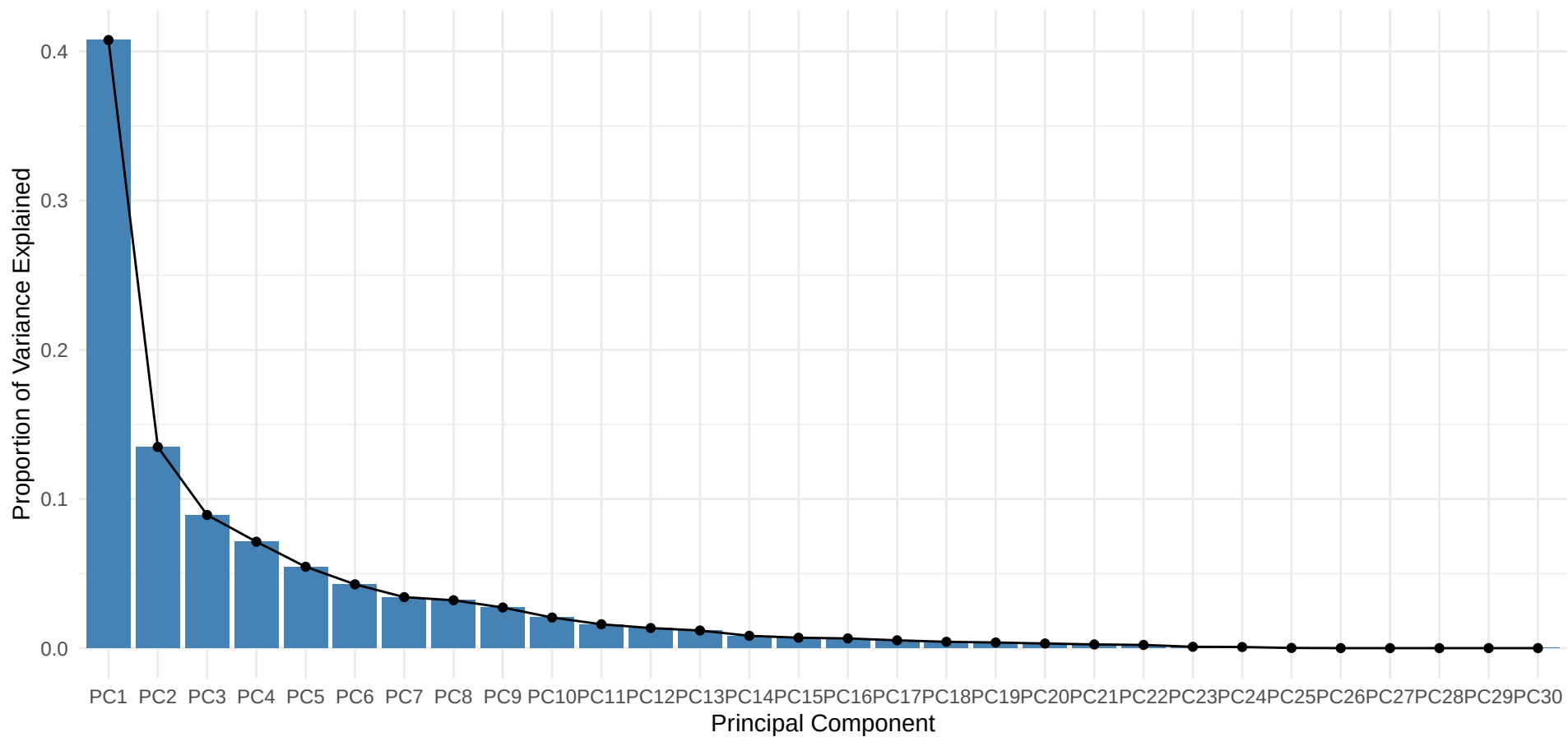
Scree Plot of PCA for FLARE005
